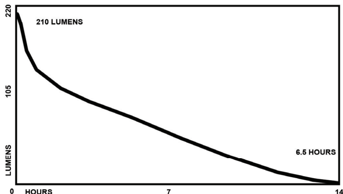
XPP-5420GX PERFORMANCE CURVE
